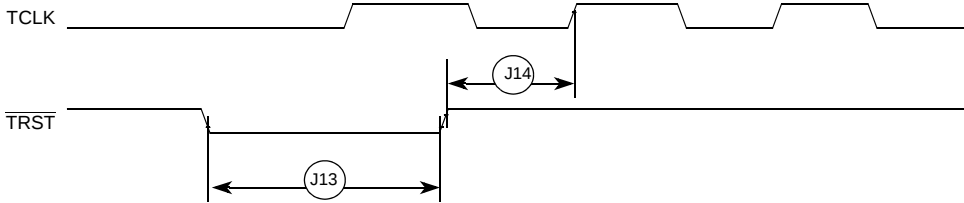
Figure 31. \overline{\text{TRST}} Timing
