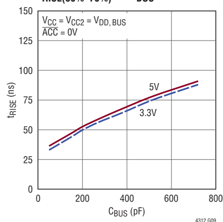
t_{RISE}(30\%-70\%) vs C_{BUS}
