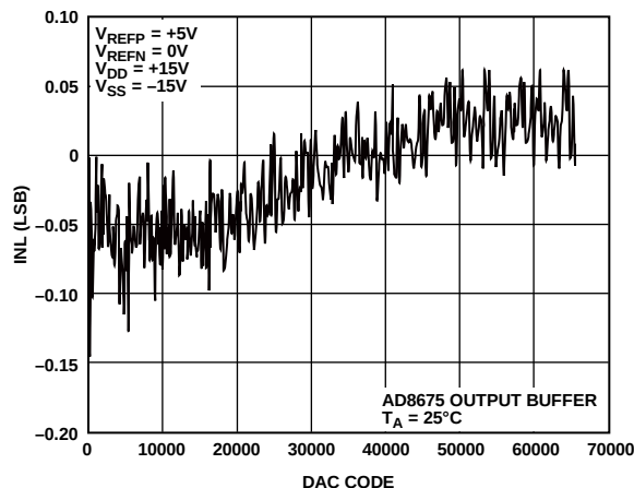
Figure 8. Integral Nonlinearity Error vs. DAC Code, 5 V Span, \times 2 Gain Mode
