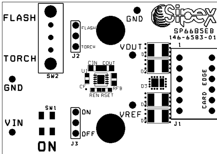
FIGURE 9: SP6686EB COMPONENT PLACEMENT
