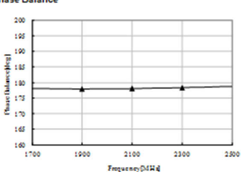
Phase Balance
