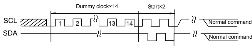
Figure 41-(a). The Case of Dummy Clock × 14 + START × 2 + Command Input
