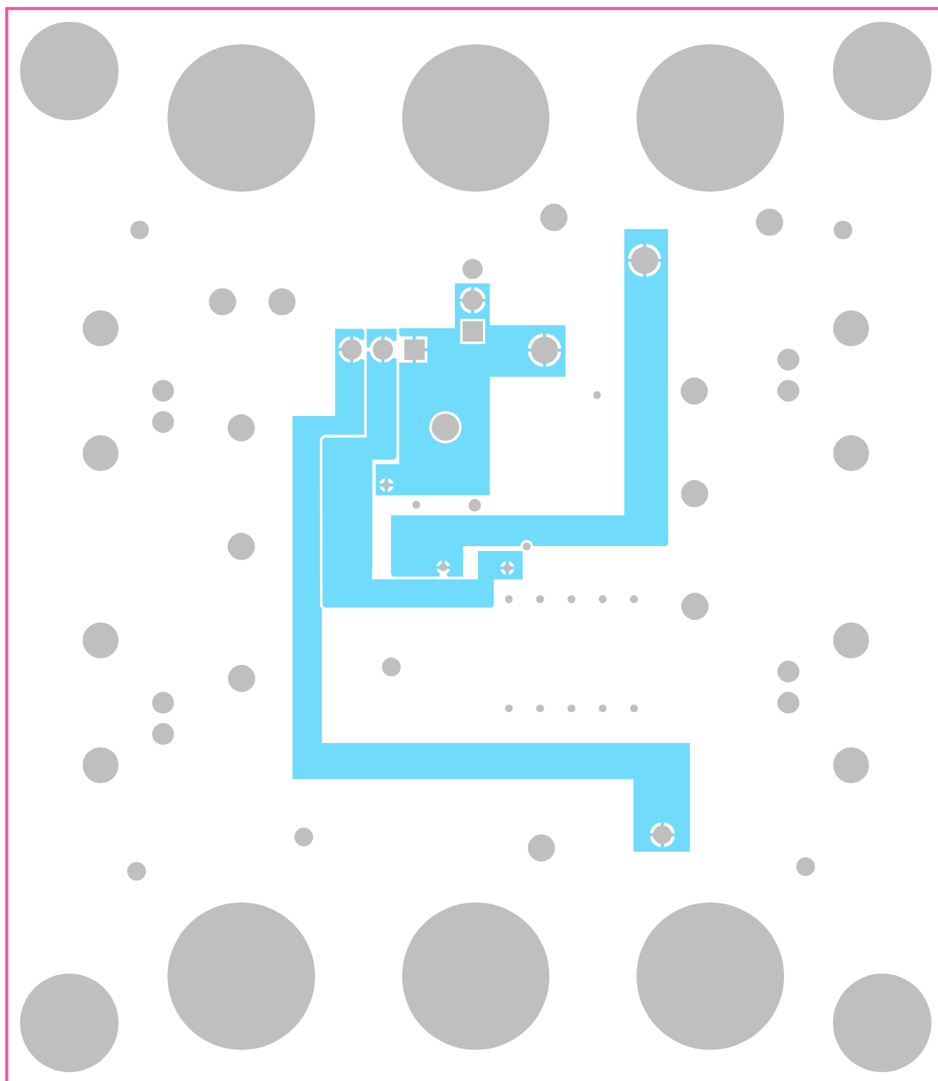
Figure 6. Layer 3 (Power)
