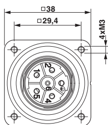
Dimensioned drawing
