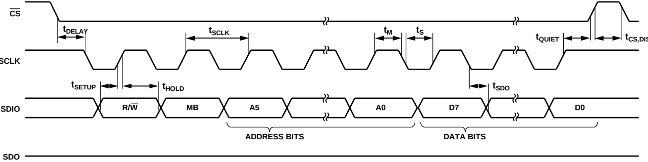
Figure 29. SPI 3-Wire Read/Write
