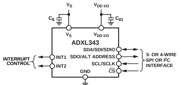
Figure 34. Application Diagram
