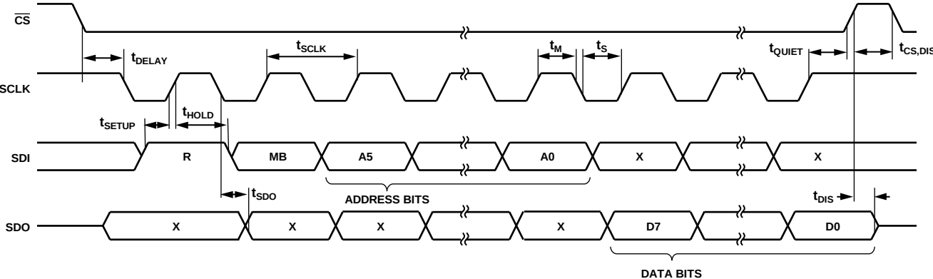
Figure 28. SPI 4-Wire Read
