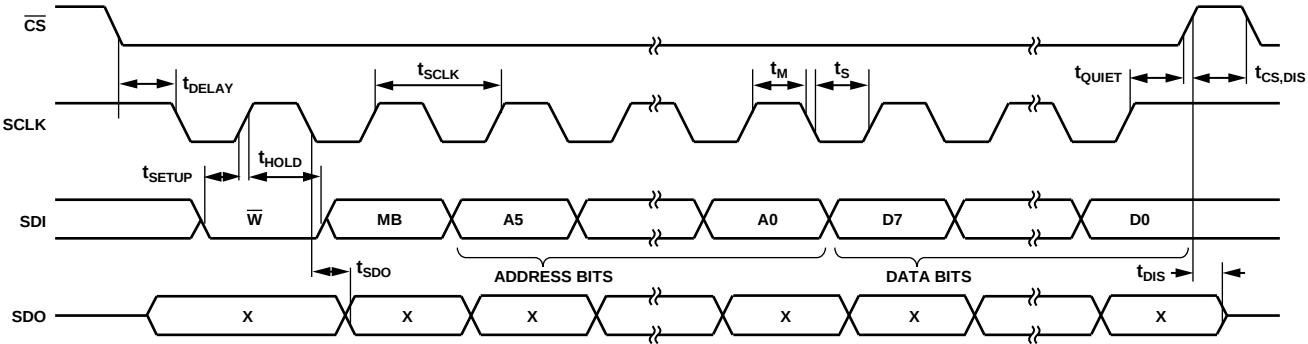
Figure 27. SPI 4-Wire Write
