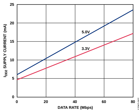
Figure 7. Typical I D02 Supply Current vs. Data Rate for 5.0 V and 3.3 V Operation
