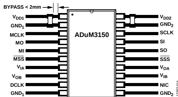
Figure 14. Recommended PCB Layout
