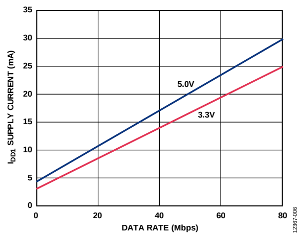
Figure 6. Typical I D01 Supply Current vs. Data Rate for 5.0 V and 3.3 V Operation
