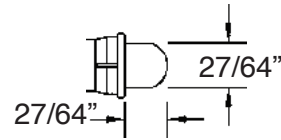
Dome Lens Style With bezel.
