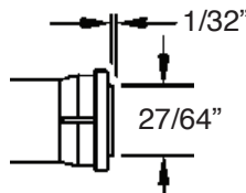
Flush Lens With bezel.
