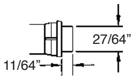
Flat Cylindrical Lens With bezel.
