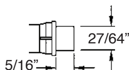
Hi-Hat Lens Style With bezel.
