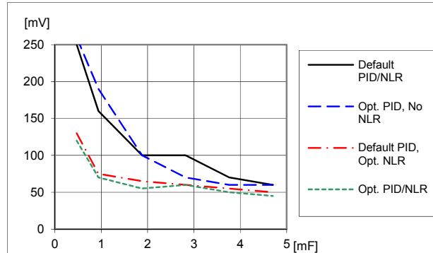
Load Transient vs. External Capacitance, V_O = 1.0 V
