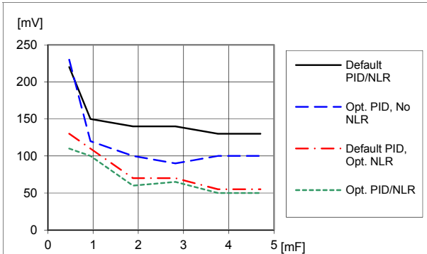
Load Transient vs. External Capacitance, V_O = 3.3 V
