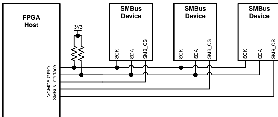
Figure 11. SMBus Configuration 2
