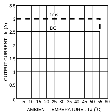
Fig.12 Derating curve
