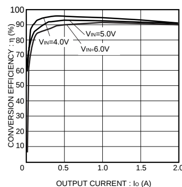
Fig.10 Conversion efficiency
