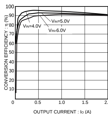
Fig.10 Conversion efficiency
