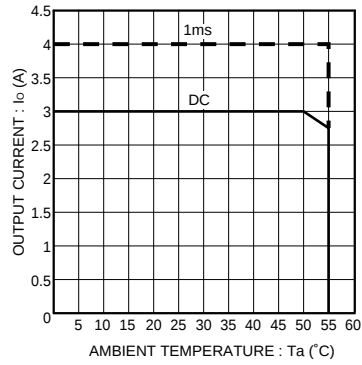
Fig.15 Derating curve
