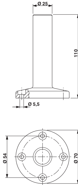
Dimensional drawing
