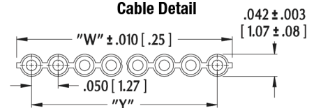
Cable Detail
