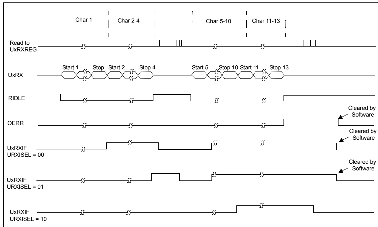
FIGURE 22-2: UART RECEPTION
