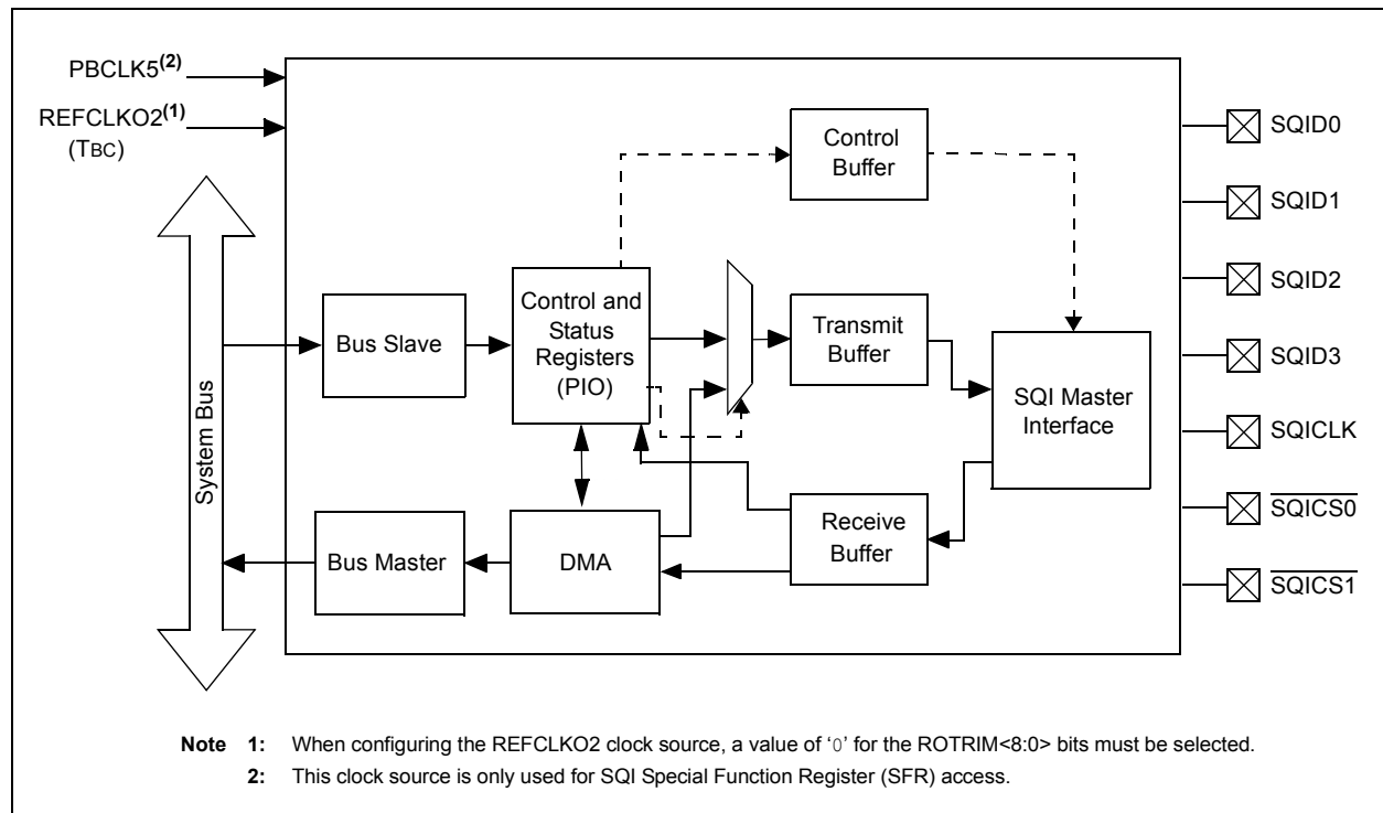
FIGURE 20-1: SQT MODULE BLOCK DIAGRAM
