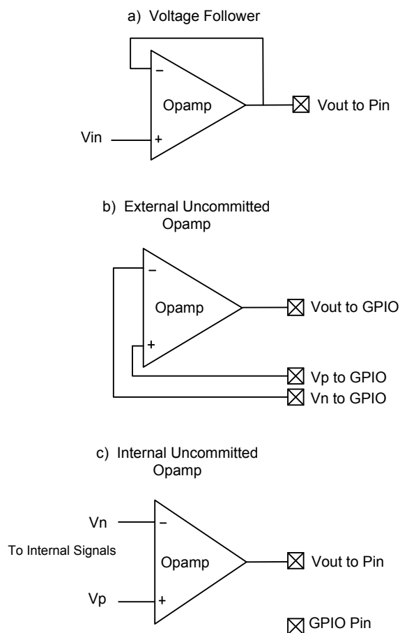
Figure 8-8. Opamp Configurations
