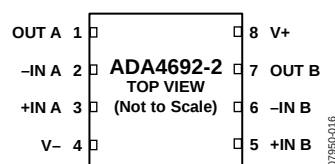
Figure 6. 8-Lead, 2 mm x 2 mm LFCSP (CP-8-6)
