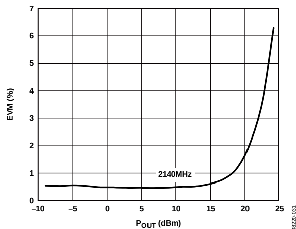
Figure 31. EVM vs. P_{OUT} at 2140 MHz
