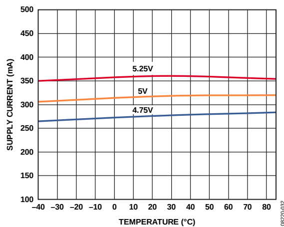
Figure 32. Supply Current vs. Supply Voltage and Temperature at 2140 MHz
