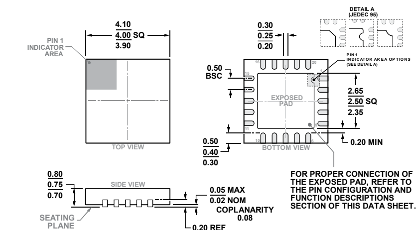
Figure 46. 20-Lead Lead Frame Chip Scale Package [LFCSP] 4 mm × 4 mm Body and 0.75 mm Package Height (CP-20-10) Dimensions shown in millimeters
