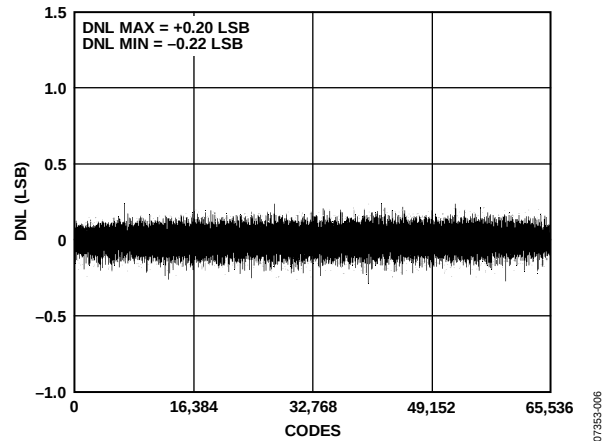
Figure 11. Differential Nonlinearity vs. Code, V_{REF} = V_{DD} = 5\text{ V}
