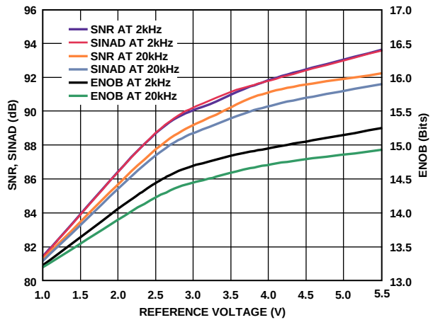
Figure 15. SNR, SINAD, and Effective Number of Bits (ENOB) vs. Reference Voltage
