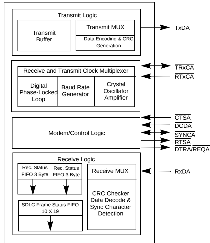
Channel A Exploded View
