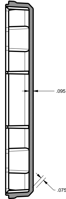
SECTION Y-Y
