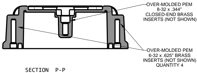
SECTION P-P
