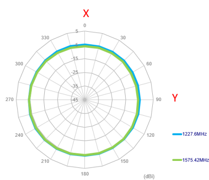
XY Plane
