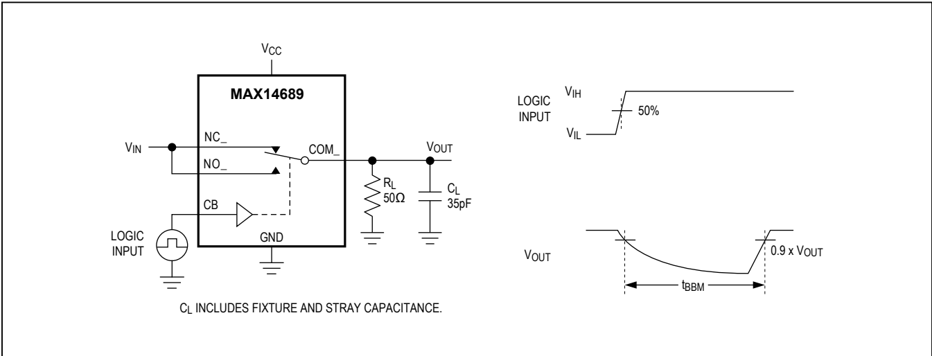
Figure 2. Break-Before-Make Interval
