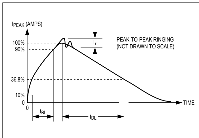
Figure 5. Human Body Current Waveform
