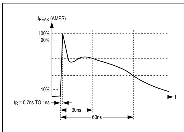
Figure 7. IEC 61000-4-2 ESD Generator Current Waveform
