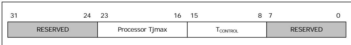
Figure 2-30. Temperature Target Read
