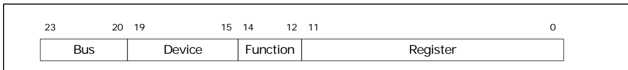
Figure 2-46. PCI Configuration Address for local accesses
