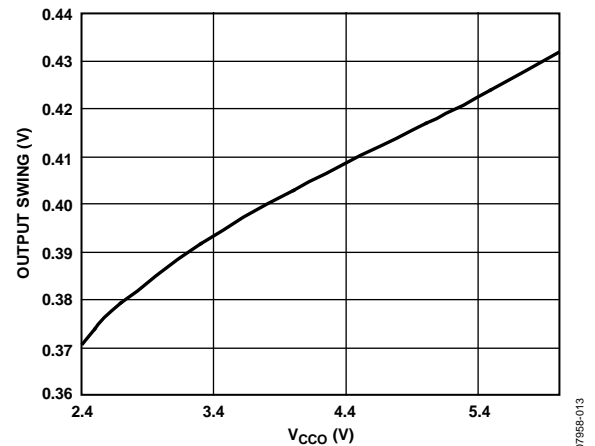
Figure 13. LVDS Output Swing vs. V_{CCO}
