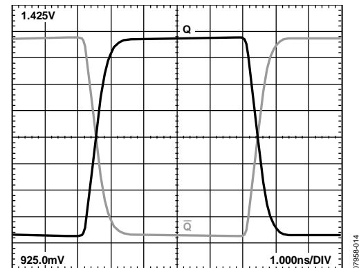
Figure 14. 50 MHz Output Voltage Waveform at V_{CCO} = 2.5\text{ V}
