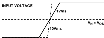
Figure 16. Propagation Delay—Overdrive Dispersion
