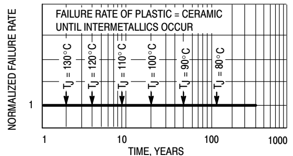
Figure 3. Failure Rate vs. Time Junction Temperature
