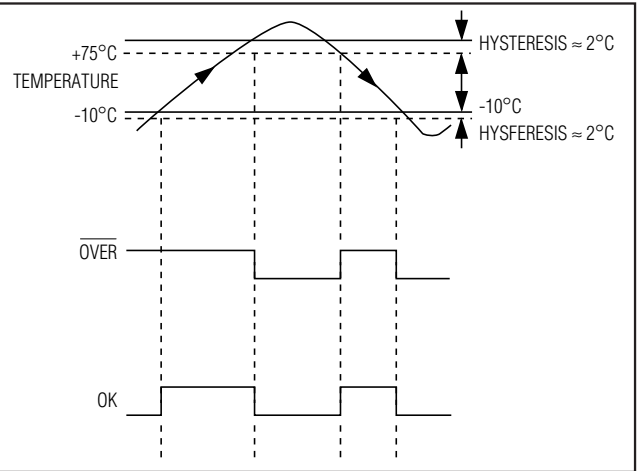
Figure 2. Temperature Response—MAX6507A04B Outputs with 2°C Hysteresis
