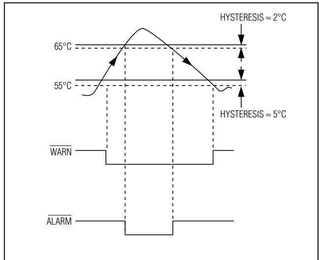
Figure 1. Temperature Response—MAX6505UTP065 Outputs, \Delta T_{\text{AW}} = 10^{\circ}\text{C} , and WARN Hysteresis \approx 5^{\circ}\text{C}
