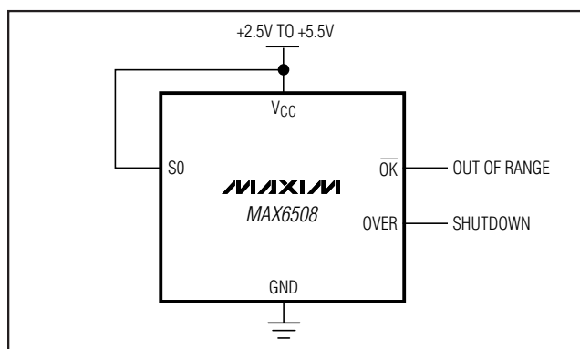
Figure 4. Temperature-Window Alarms
