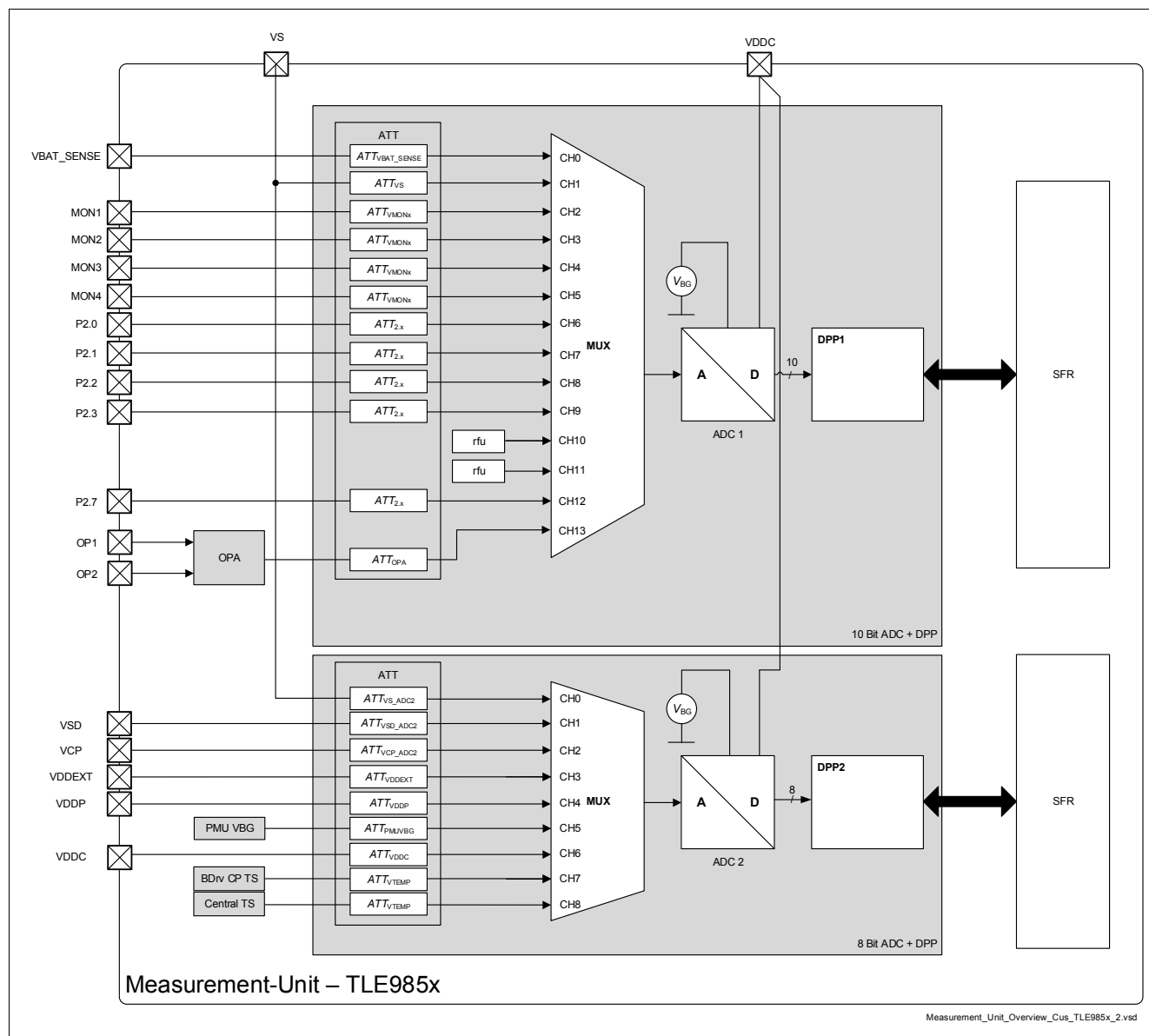
Figure 28 Measurement Unit-Overview
