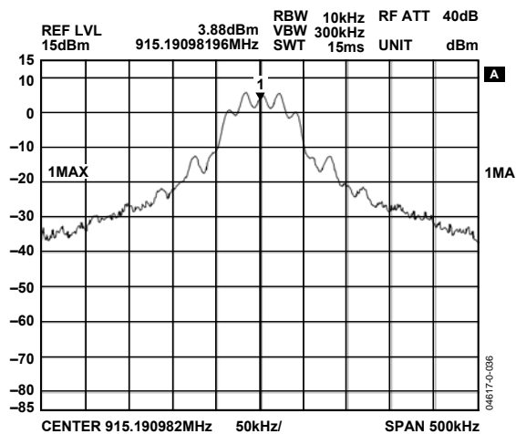
Figure 22. FSK Modulation, Power = 10 \text{ dBm} , Data \text{ Rate} = 38.4 \text{ kbps} , F_{DEVIATION} = \pm 19.2 \text{ kHz}
