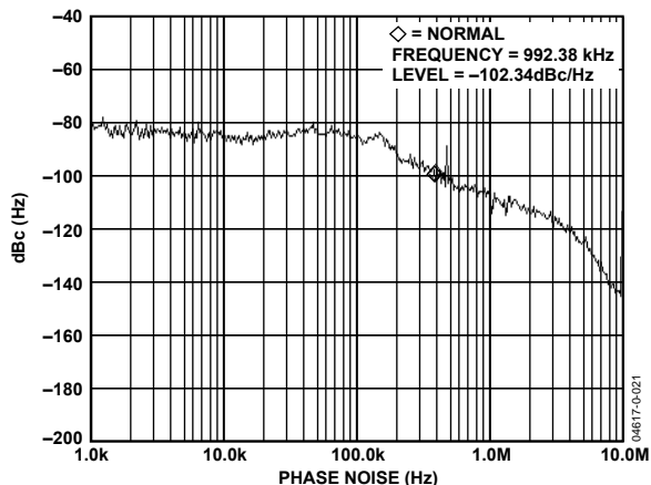
Figure 21. Phase Noise Response— I_{CP} = 1.44 \text{ mA} , I_{VCO} = 3.0 \text{ mA} , R_{FOUT} = 915.2 \text{ MHz} , PFD = 10 \text{ MHz} , Power = 10 \text{ dBm} , PA \text{ Bias} = 5.5 \text{ mA}
