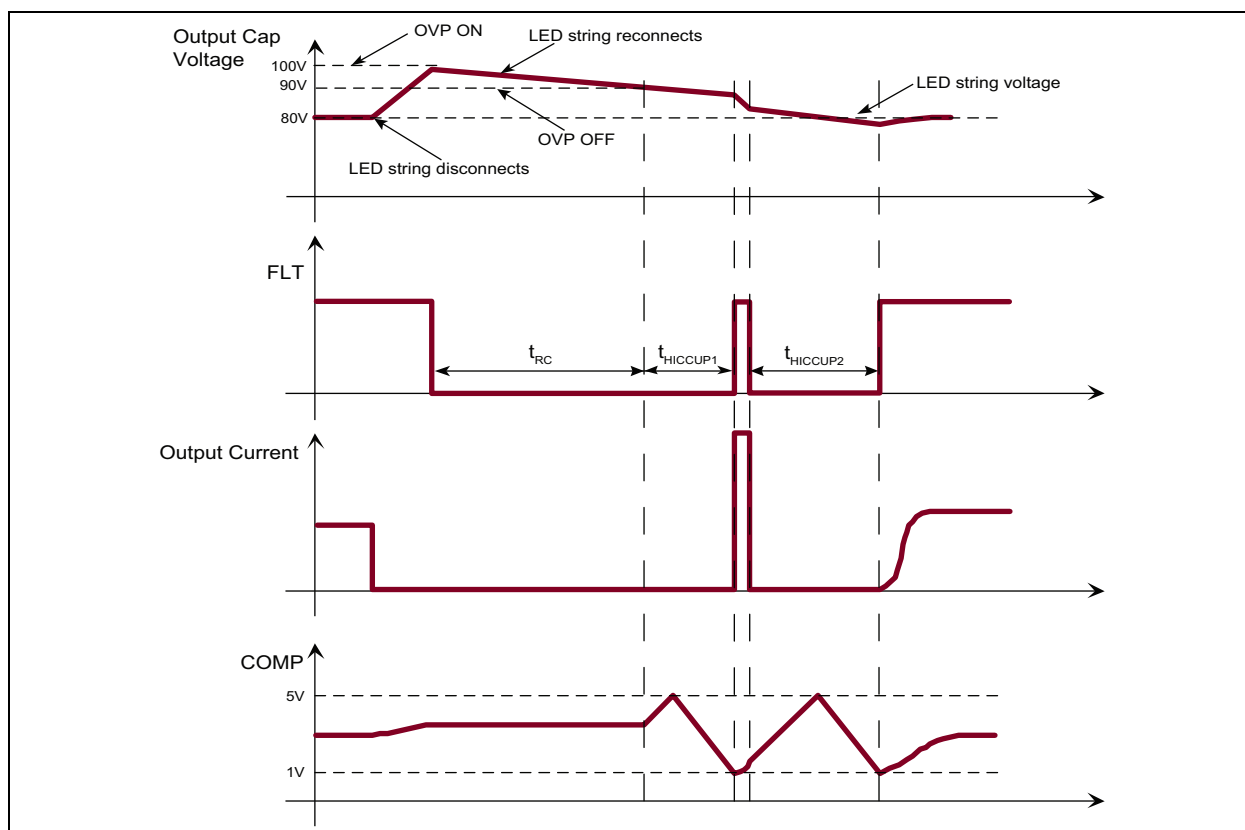
FIGURE 3-4: Open-circuit Protection.
