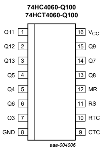
Fig. 5. Pin configuration SOT109-1 (SO16), SOT338-1 (SSOP16) and SOT403-1 (TSSOP16)
