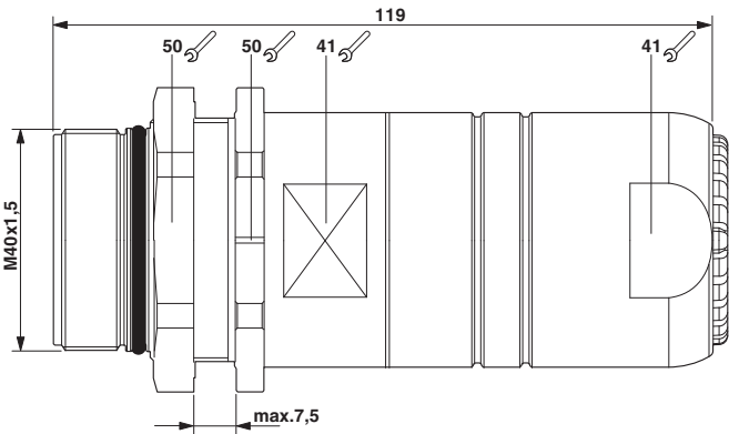
Dimensioned drawing
