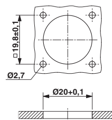
Dimensional drawing
