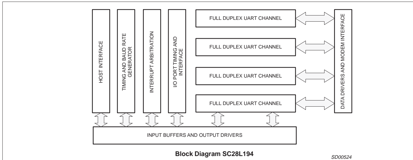
Figure 2. Block Diagram
