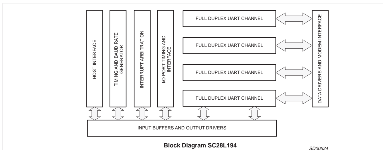
Figure 2. Block Diagram
