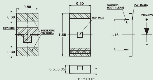
Top View Chip LED (0603/0.3T) 1.60(L) x 0.8(W) x 0.3(H)mm
