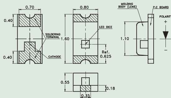
Top View Chip LED (0603/0.55T) 1.6(L) x 0.8(W) x 0.55(H)mm
