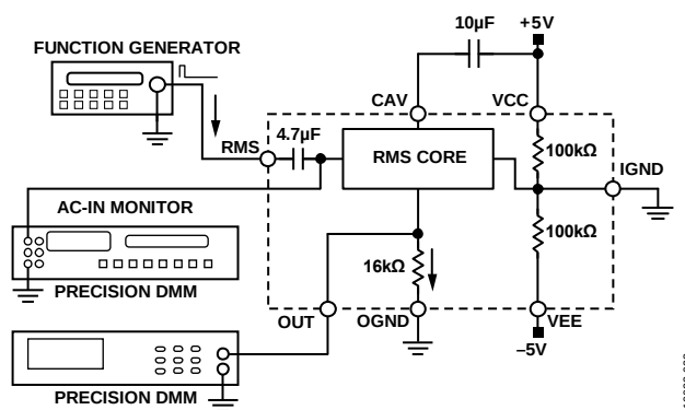
Figure 23. Crest Factor Test Circuit
