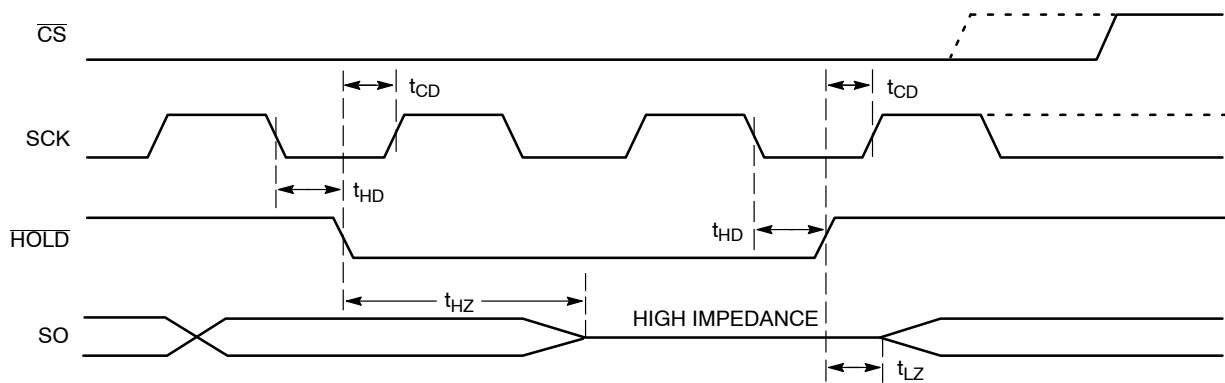
Figure 11. \overline{\text{HOLD}} Timing
