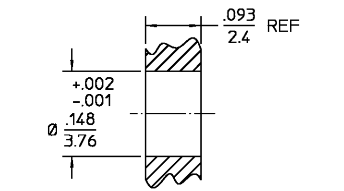
RECOMMENDED MOUNTING HOLE FOR SOLDER APPLICATIONS ONLY
