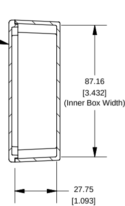
SECTION A-A End View of Assembly
