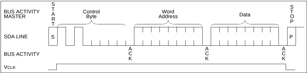
FIGURE 4-2: BYTE WRITE
