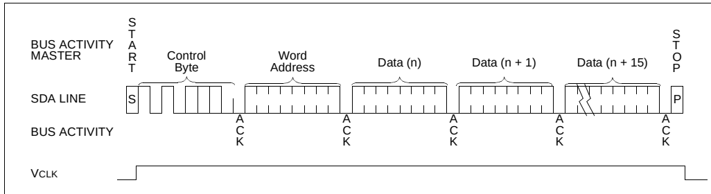
FIGURE 4-3: PAGE WRITE
