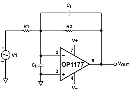
Figure 60. Compensation Using Feedback Capacitor
