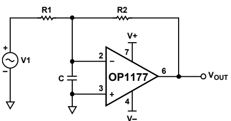
Figure 61. EMI Reduction
