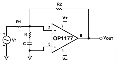
Figure 62. Compensation Using Input R-C Network
