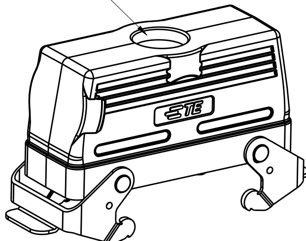
TYPE 2: LOW CONSTRUCTION, TOP ENTRY WITH STEEL DOUBLE LOCKING OTHER SPEC REFER TO TYPE 1
