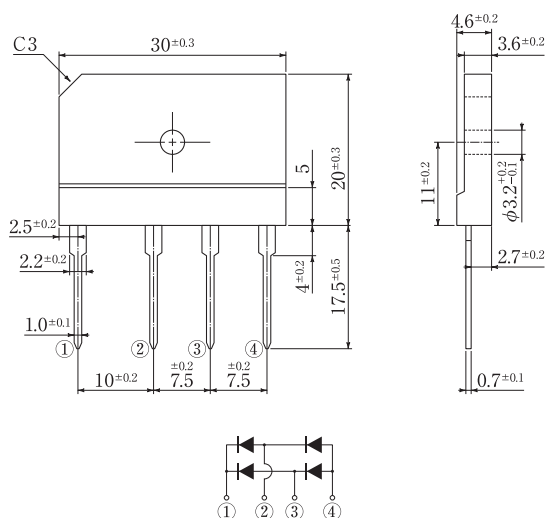
Fig.58 Package: 5S
