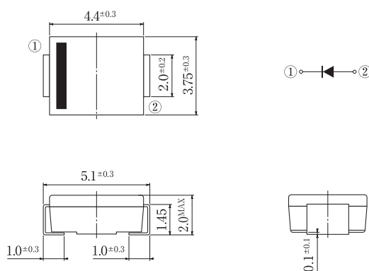
Fig.15-1 Package: M2F
