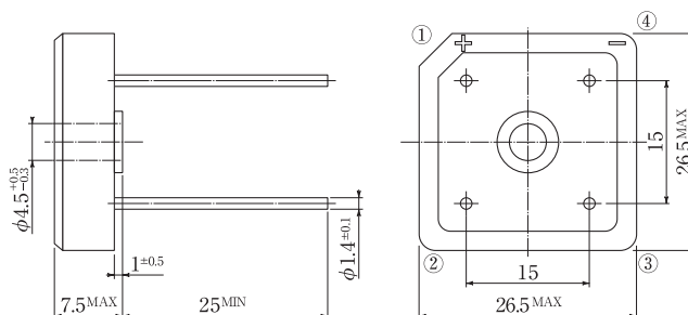
Fig.70 Package: S15WB
