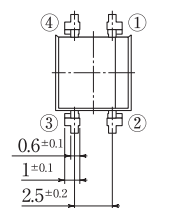
Fig.21 Package: 1Y
