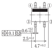
Fig.23 Package: 1Z
