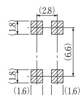
Fig.23 Package: 1Z
