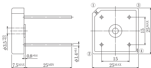
Fig.63 Package: S5VB
