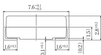
Fig.22 Package: 1Y
