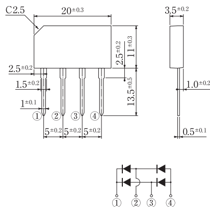
Fig.56 Package: 2S
